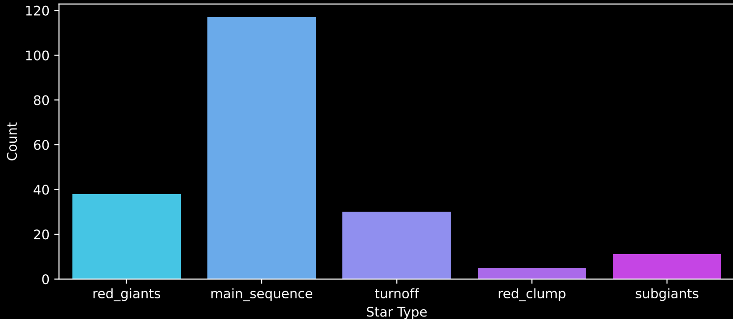
APOGEE DR17 Field: [K2_C5_212+30_btx] Count plot of Star Type
