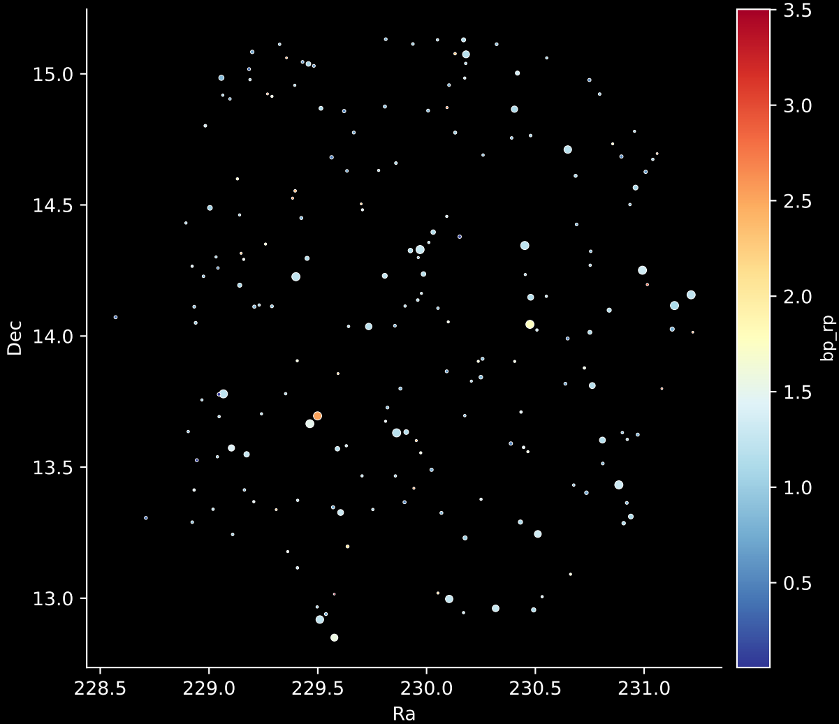
APOGEE DR17 Field: [K2_C5_212+30_btx] Stars: 201
