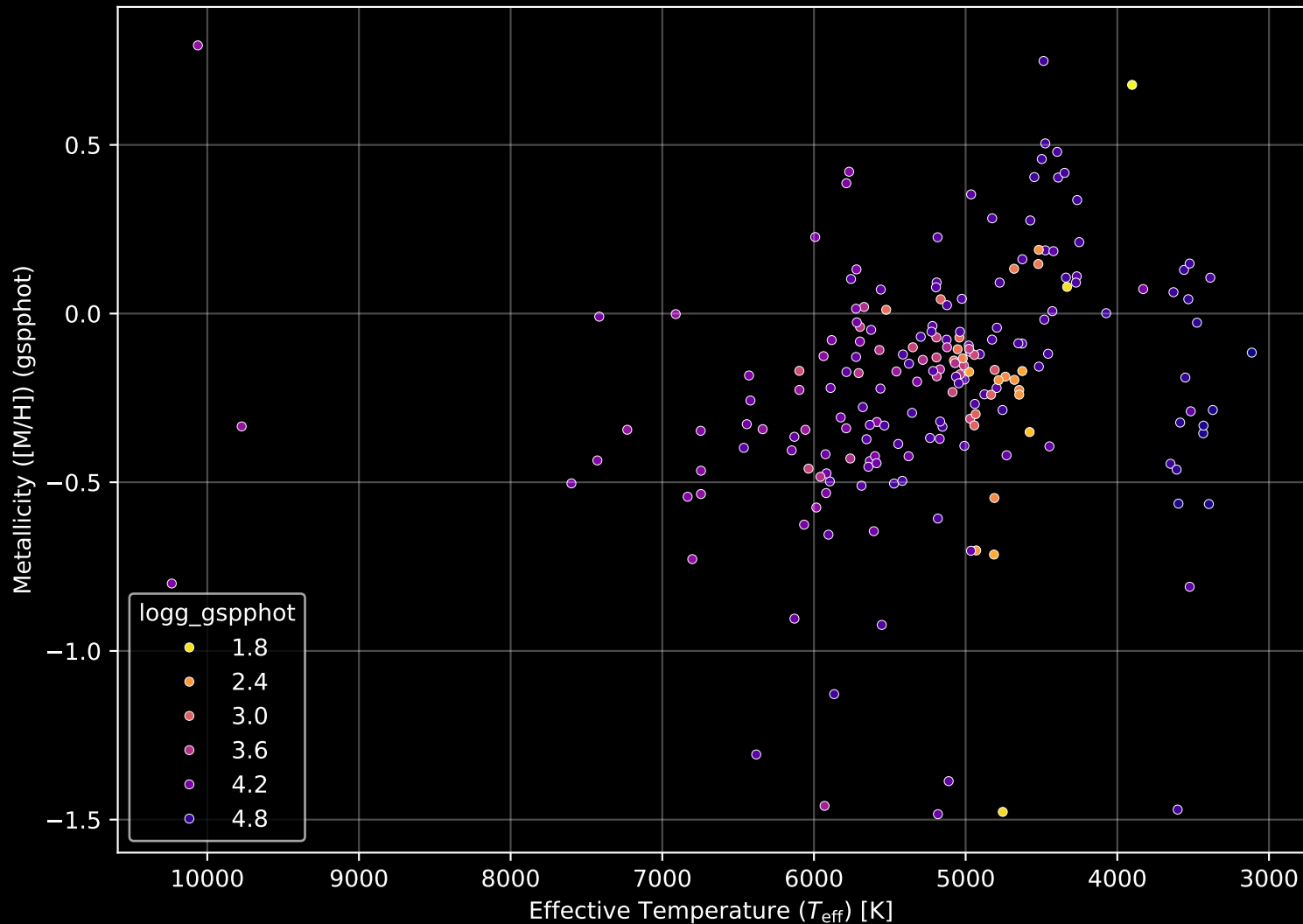
APOGEE DR17 Field: [K2_C5_212+30_btx] Stellar Population Parameters (n= 201)
