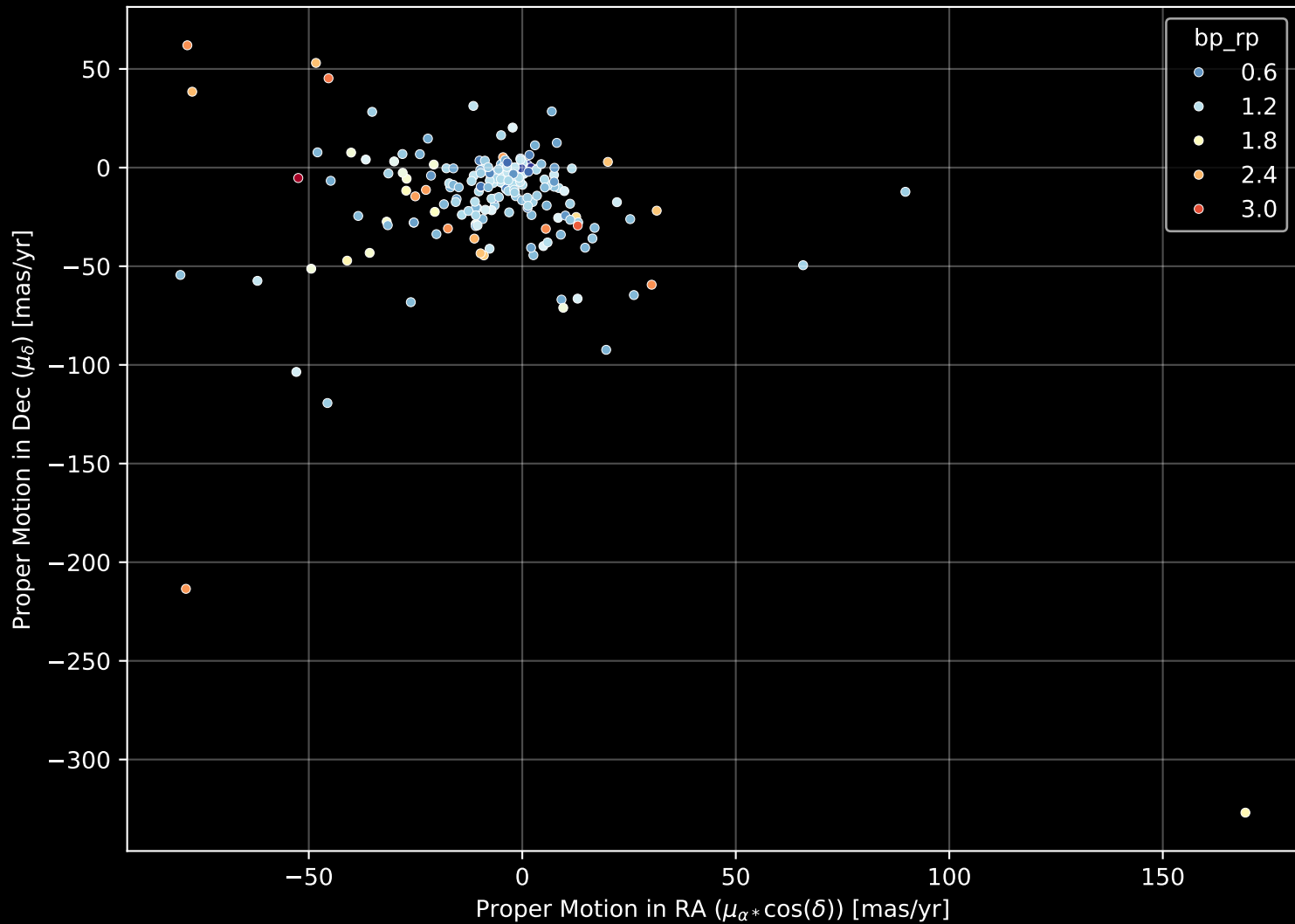
APOGEE DR17 Field: [K2_C5_212+30_btx] Proper Motion Diagram (n= 201)
