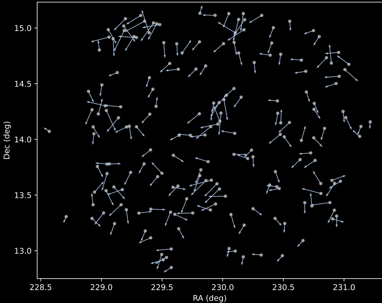
APOGEE DR17 Cluster 1 Proper Motion Vectors (n=183)
