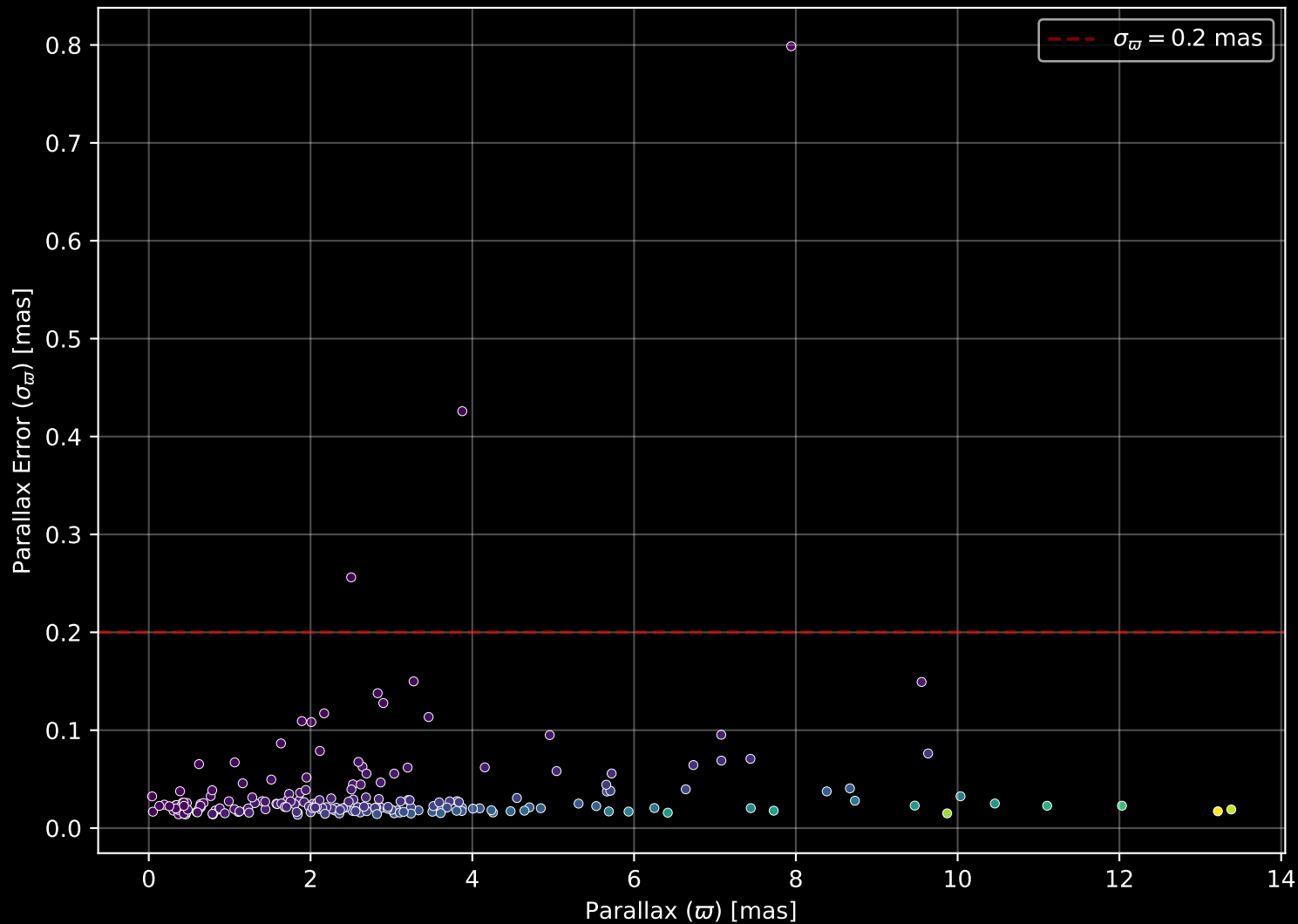
APOGEE DR17 Field: [K2_C5_212+30_btx] Parallax Quality (n= 201)
