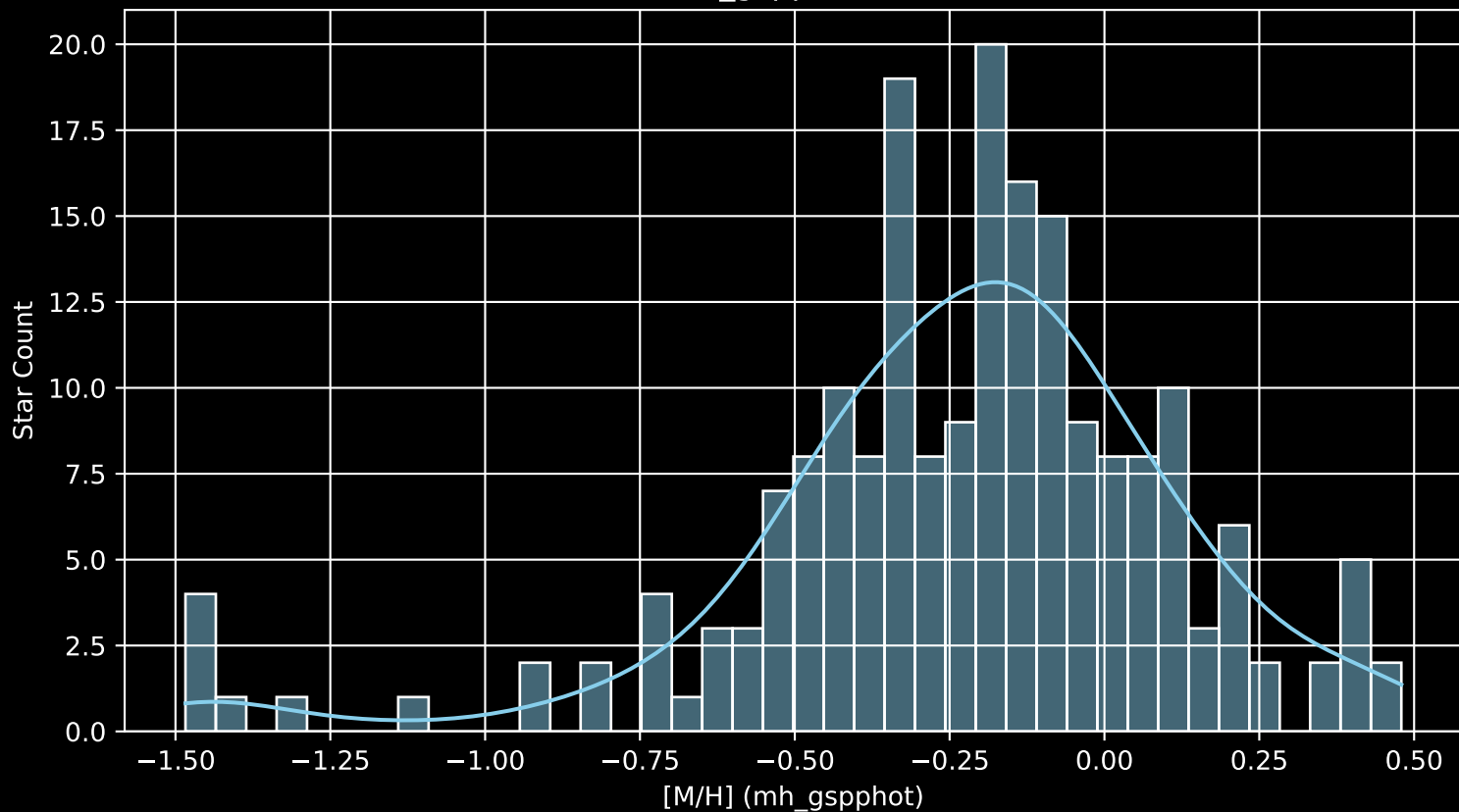
APOGEE DR17 Field: [K2_C5_212+30_btx [M/H] (mh_gspphot) (n= 197)
