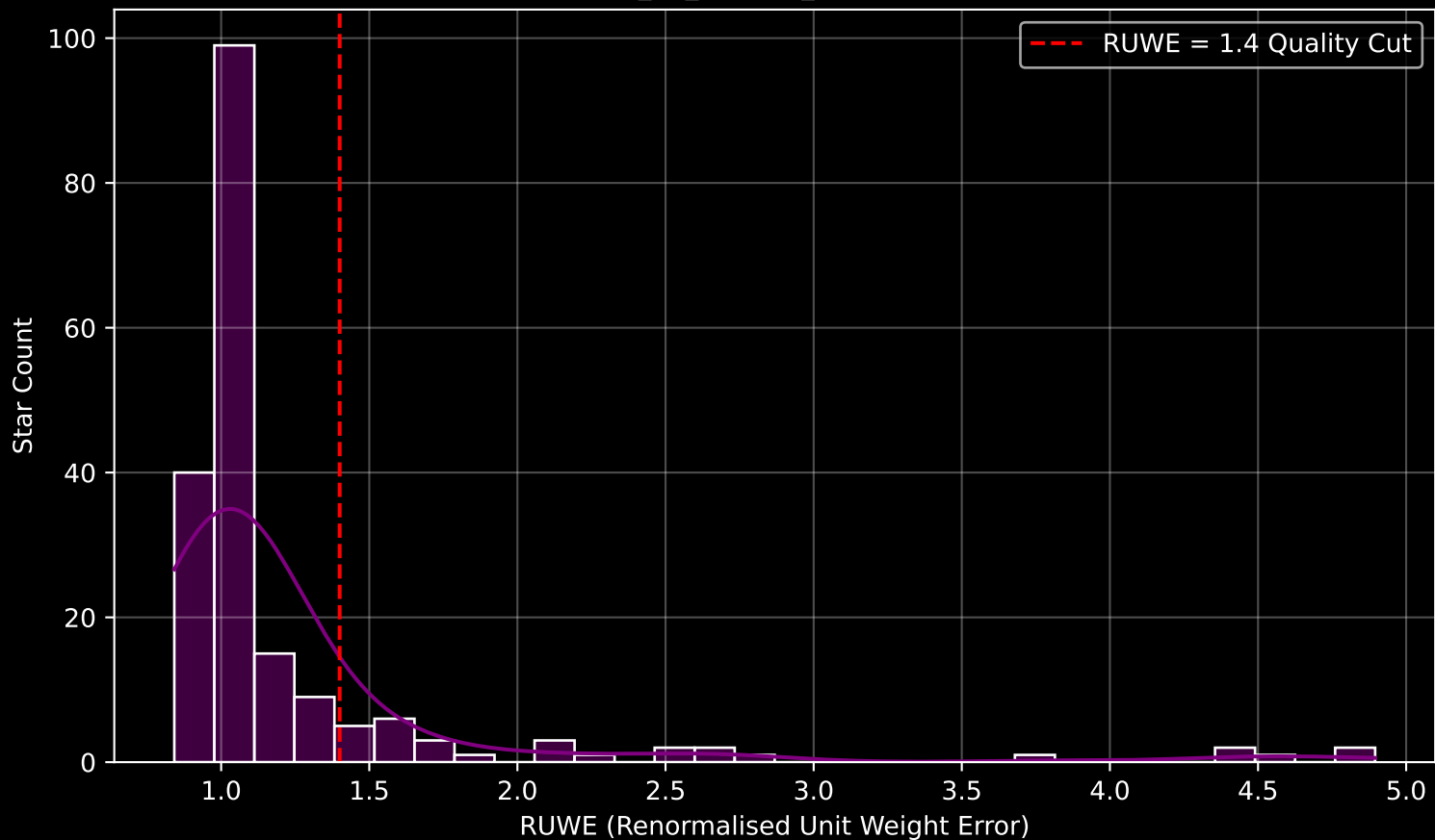
GAPOGEE DR17 Field [K2_C5_212+30_btx] RUWE Distribution (n= 193)
